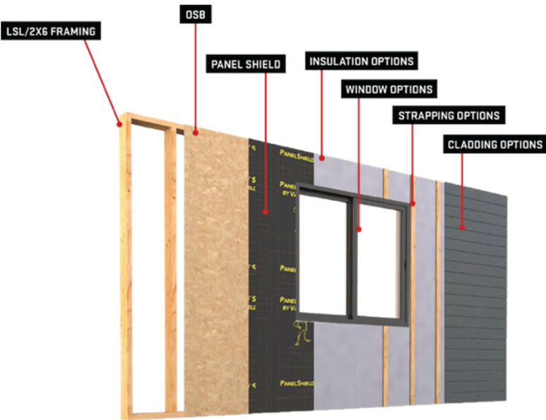
Assembly diagram: PrimePanel PH-FR representative assembly showing LSL/2×6 framing core, project-specified sheathing, WRB membrane, continuous insulation, strapping, window integration, and cladding system. ***OSB and cladding shown are for illustrative purposes only; alternate sheathing, insulation, and cladding options are available based on project requirements***
